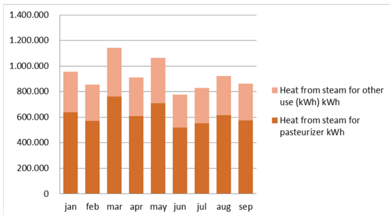
Figure 2. Monthly distribution of thermal consumption for steam production divided into; thermal energy for steam used in pasteurizers and steam used in the remaining thermal users of the production lines
