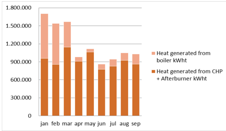
Figure 4. Total monthly thermal energy produced consumed by the plant and divided into thermal energy produced in the boiler and thermal energy produced by the CHP + Post Combustor (values expressed in thermal kWh)
