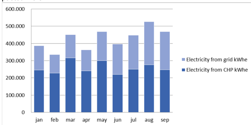
Figure 3. Total monthly electricity consumed divided into: produced by the CHP and purchased from the grid
