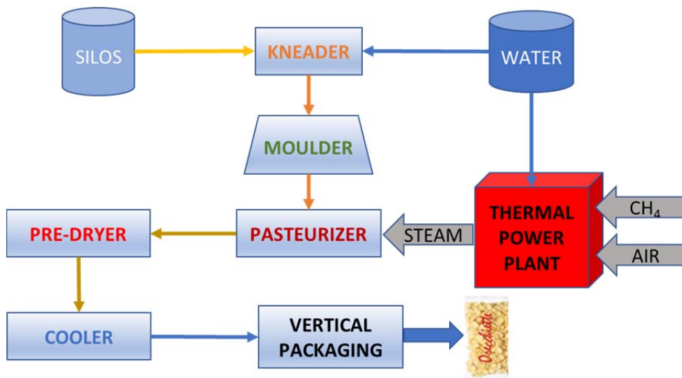
Figure 1. Total mass balance of the fresh semolina pasta production line
