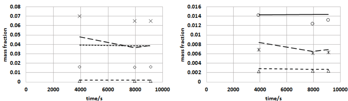
Figure 3 a, b: Mass fraction of minor components in organic (left) and aqueous (right) phase of distillate. MIBK, O and solid line; water, ◇ and square dot; acetic acid, △ and dash; furfural, x and long dash. Average uncertainty of measured mass fraction is 0.002.
