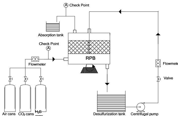
Figure 1: The experimental flow chart of selective absorption of H 2 S
