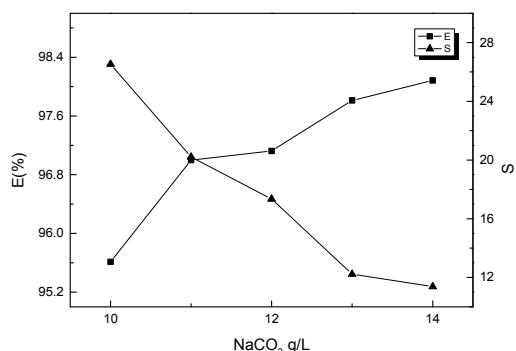
Figure 6: Effect of alkali concentration on selectivity
