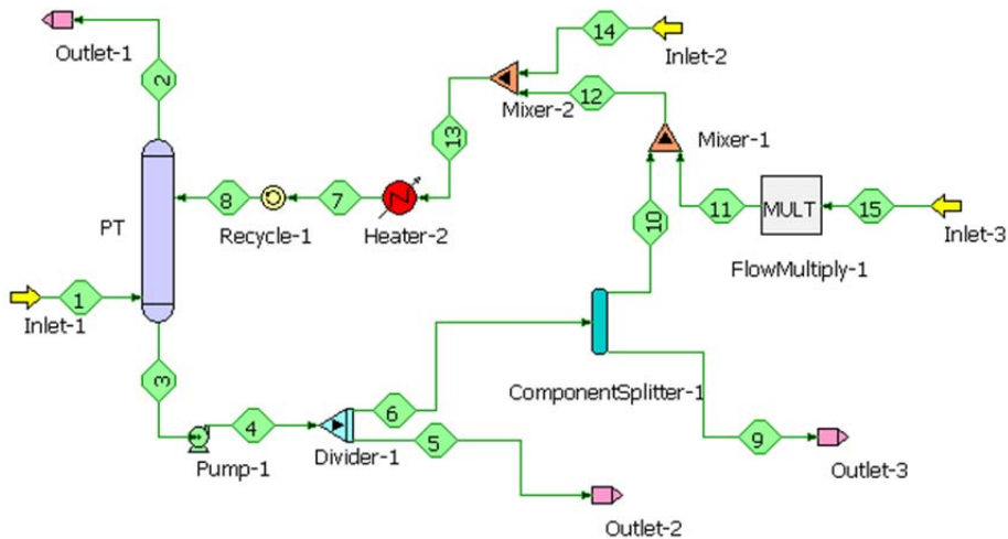
Figure 1: ProTreat model of the CS-Cap process SO 2 capture loop
