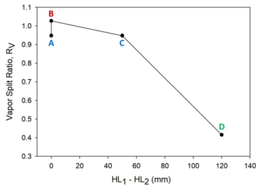
Figure 6: Summary of a case study during DWC operation: (A) Design, (B) Without EAVD ® , (C) EAVD ® adjust the same R_V as designed, and (D) EAVD ® adjust to supply more vapor in section 2.
