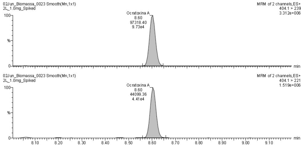
Figure 1: Chromatogram (UPLC) of extract from culture medium 2 fortified with OTA.
