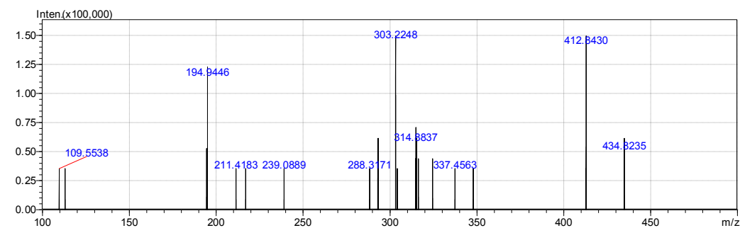
Figure 3: Mass spectrum of the extract from culture medium 2.
