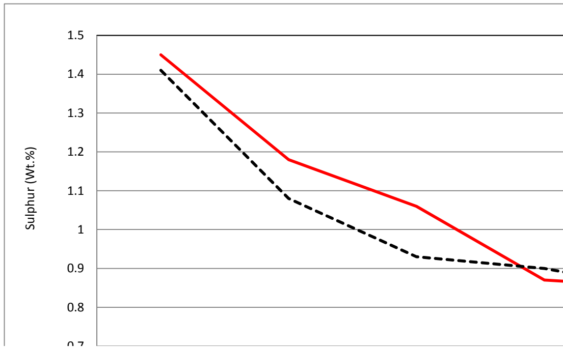
Figure 1: Variation of sulphur content with HRTs
