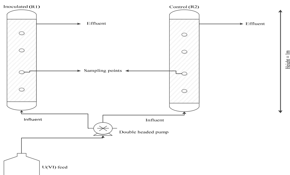
Figure 1: Continuous-flow system laboratory set
