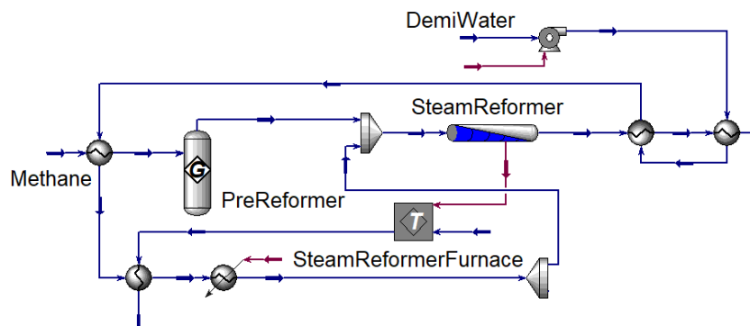
Fig.3: Example of modeling for a project solution. Here it is shown the steam reforming – a method for producing syngas (hydrogen and carbon monoxide) by reaction of hydrocarbons with water.
