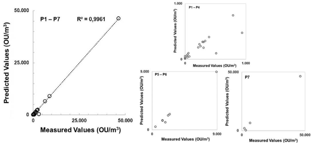
Figure 2: Correlation between the odour concentrations measured by DO and predicted by ANN referred to all data (figure on the left) and to defined sources (figures on the right).
