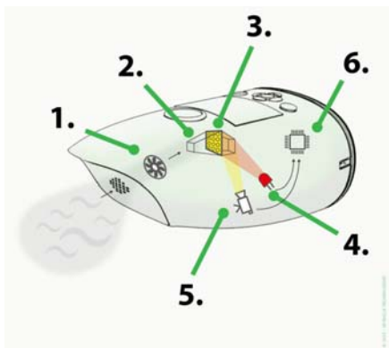
Figure 2: General principle of NeOse: 1- Pumping of air and odorous molecules; 2- Transport of compounds to the chamber; 3- Interaction of compounds with chemical sensors arrayed on a prism; 4-Lighting the prism with LED lamp; 5- Recording optical signal transduction with a camera; 6- Storage (database) and analysis results
