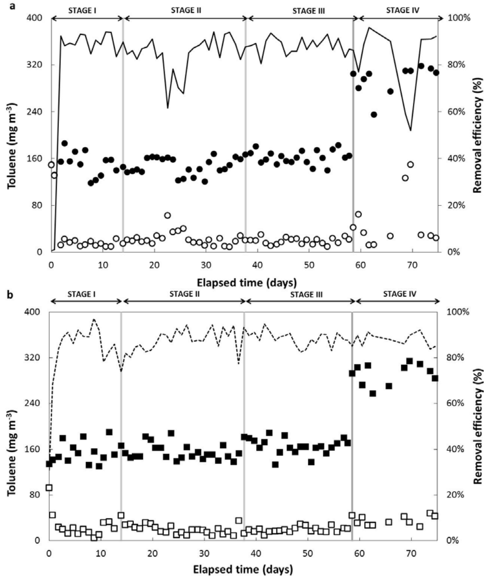
Figure 2: Time course of the inlet (dark symbols) and outlet (white symbols) toluene concentration and toluene removal efficiency (continuous line) in (a) BTF and (b) TPBR. Vertical lines represent the different operating stages as indicated in the upper part of the graphs.
